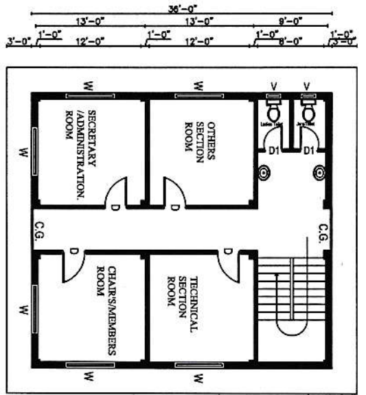
GROUND FLOOR PLAN PLINTH AREA: 1188 SQFT SCALE: 1"=8'-0"
