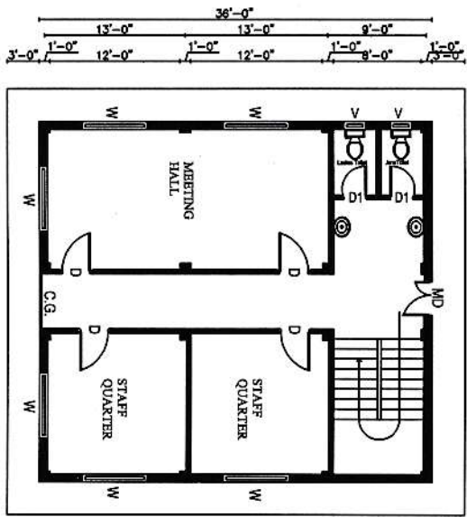
FIRST FLOOR PLAN PLINTH AREA: 1188 SQFT SCALE: 1"=8'-0"
